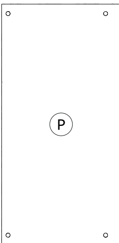
PI07995 864x429x22mm
