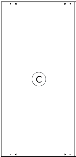
CA04232 912x447x22mm
