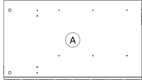
FI10092 780x445x22mm
