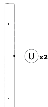
FS05274 676x60x22mm
