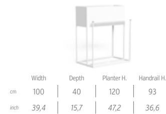
PLANTER+HANDRAIL H120/ CODE: PAT120H
