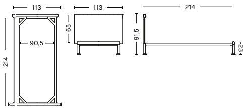
FOR MATTRESS W90 CM WIDTH 113 CM LENGTH 214 CM HEIGHT 91,5 CM
